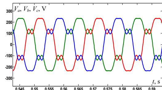
Fig. 6. Utility voltages source under harmonics
