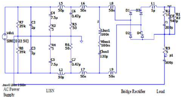
Fig. 11. Diagram of a single-phase diode rectifier with the LISN under LTspice software
