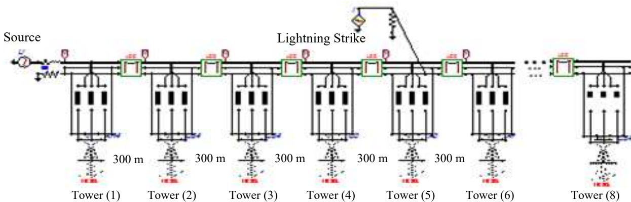
Fig. 5. The OAT-EI Hassi line (220 kV) subjected to a 1200 kV overvoltage
