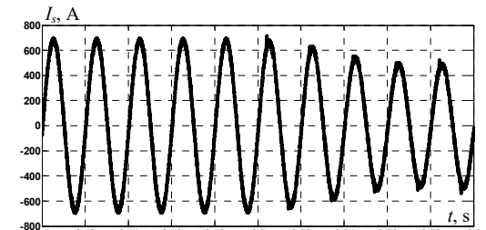
Fig. 18. Current source after filtering
