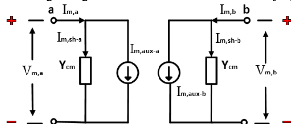
Fig. 2. Principle scheme of J.R. Marti model
