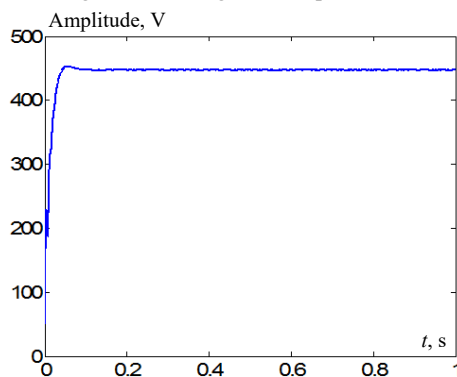
Fig. 8. Output DC voltage obtained from converter
