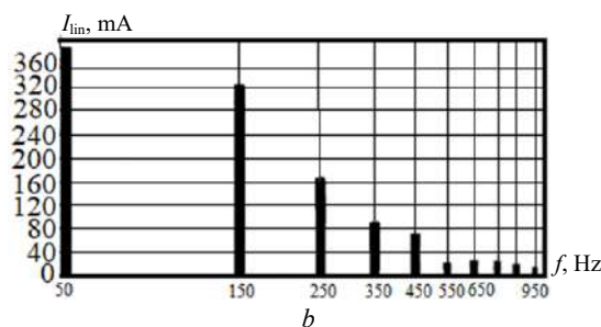
Fig. 8. Line current spectrum: a) simulation results; b) experimental results
