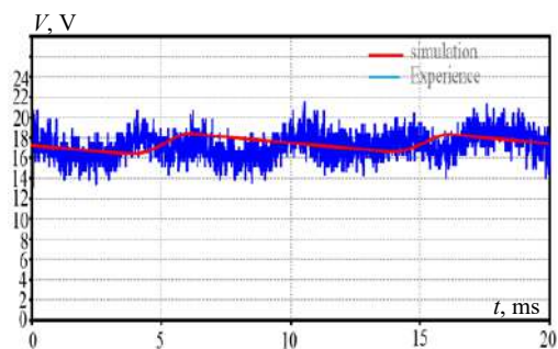
Fig. 9. Rectified voltage at the terminals of the load
