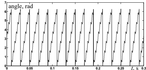
Fig. 7. Angular position estimated by the PLL based on PI controller
