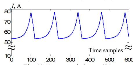
Fig. 11. Current at inductor ( L_r )
