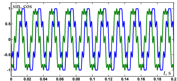
Fig. 8. Sin and cos generated by the PLL based on PI controller angle
