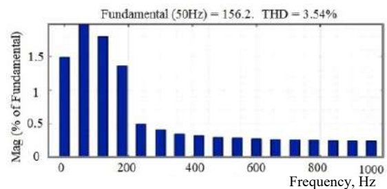
Fig. 19. Current harmonic
