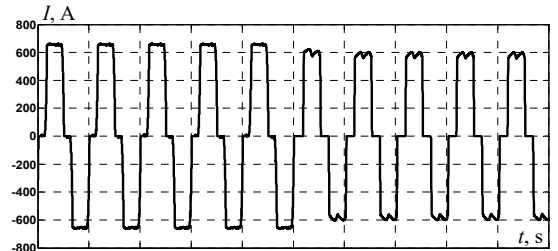
Fig. 16. Current before filtering
