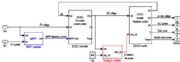
Fig. 11. Solar PV model
