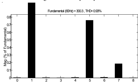
Fig. 18. THD analysis
