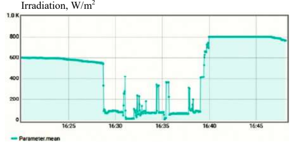
Fig. 21. Monitored irradiance in shading effect
