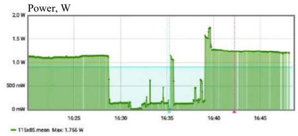
Fig. 20. Monitored PV power under shading effect
