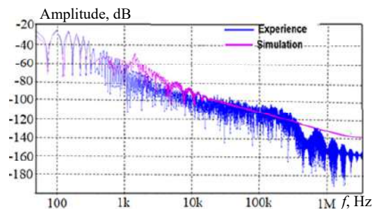
Fig. 13. I_{CM} common mode current spectrum
