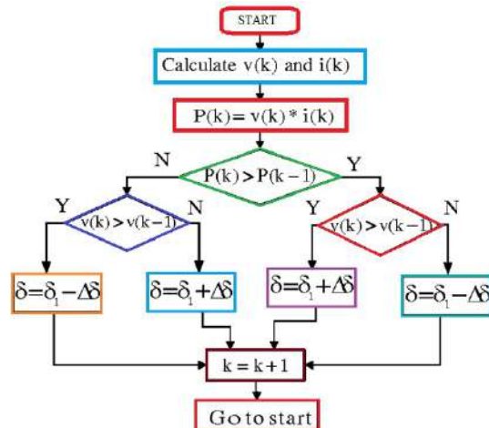
Fig. 6. P&O flowchart
