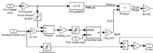
Fig. 12. Wind turbine model
