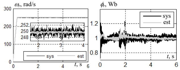
Fig. 16. Estimated speed and rotor flux
