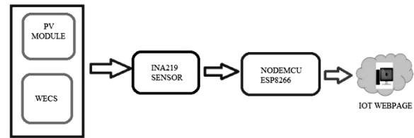
Fig. 8. Power monitoring system using IoT
