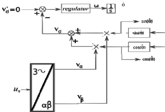
Fig. 5. Block diagram of PLL
