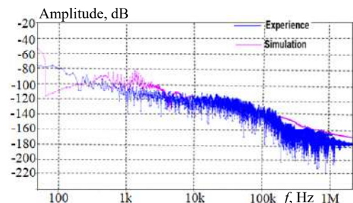
Fig. 12. Spectrum of localized differential disturbances on LISN
