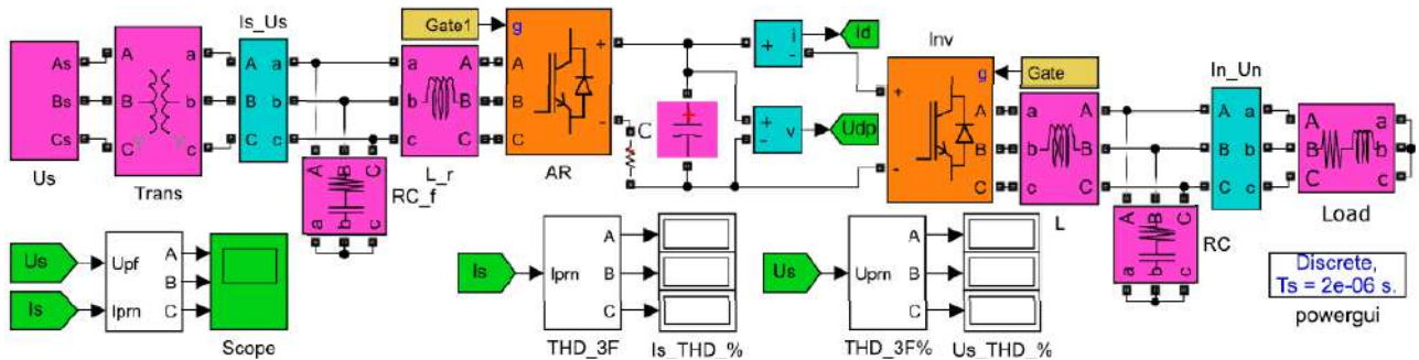
Fig. 11. MATLAB model of the ARVS power circuit
