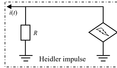
Fig. 4. Heidler type model
