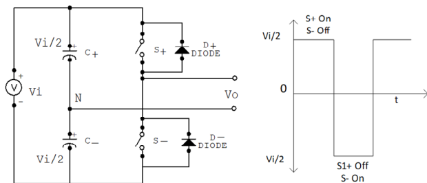
Fig. 7. Single-phase inverter
