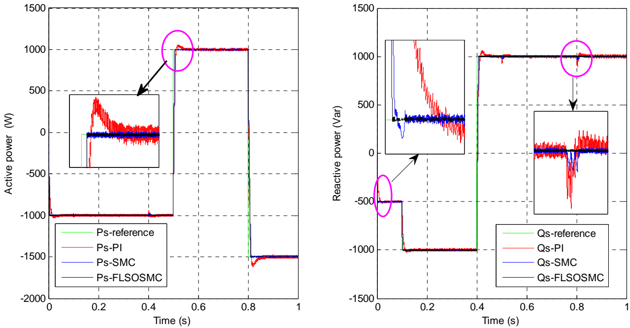
Fig. 9. Sensitivity to the reactance variation ( X_L -30\% )
