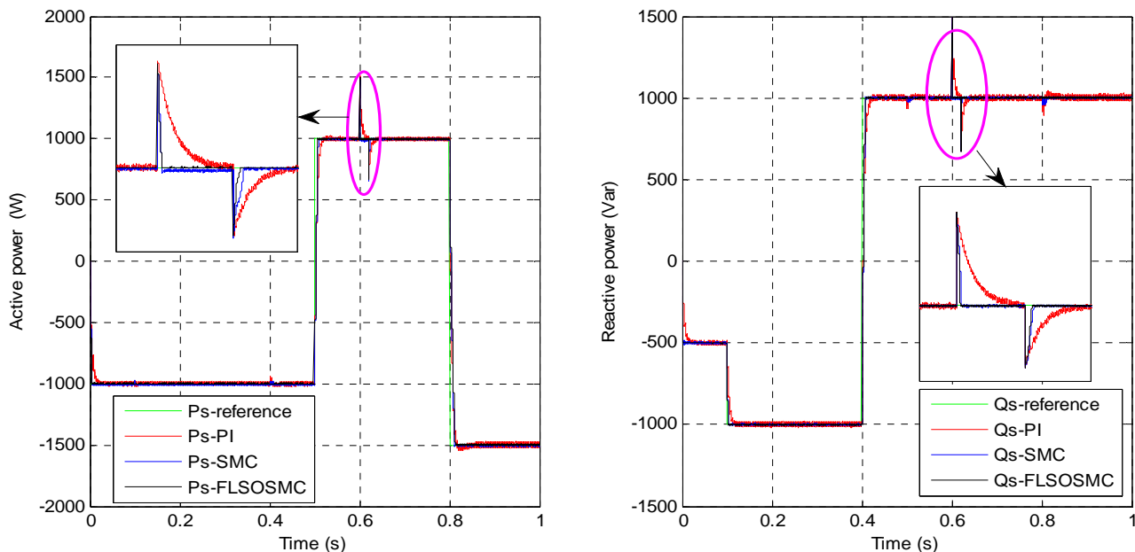
Fig. 10. Sensitivity to sub-voltage perturbation (+50 %)
